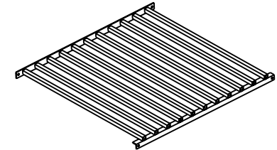
BOTTOM 10 DOOR DIVIDER WELDMENT TDFG-15479 WITH CAPS IN TUBES QTY: 1
